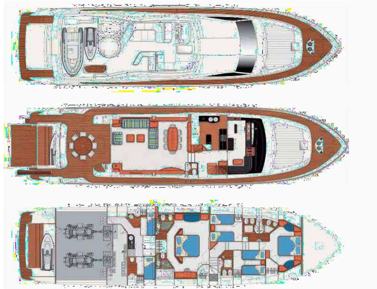
General arrangement
